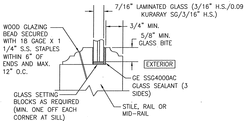
TYPICAL GLAZING DETAIL (MONOLITHIC GLASS)
