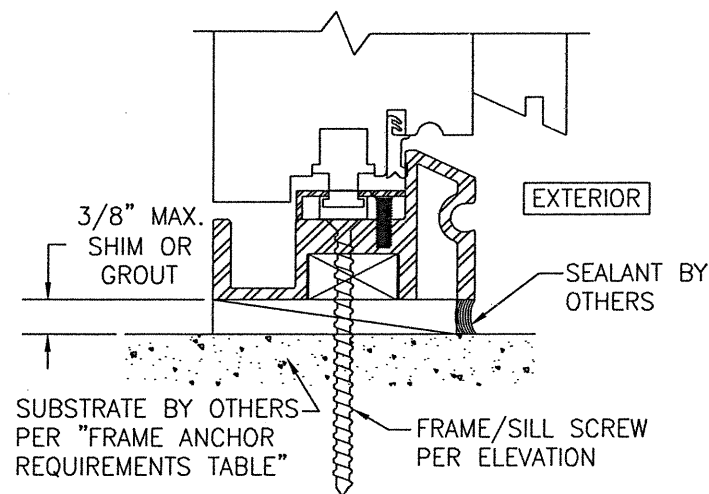
OPTIONAL FRAME SCREW MOUNT DETAIL AT SILL (NOT APPLICABLE WITH FIXED PANEL DOORS)
