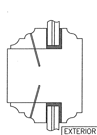
SECTION J SCALE: 1/2 FULL (GLASS OVER GLASS)
