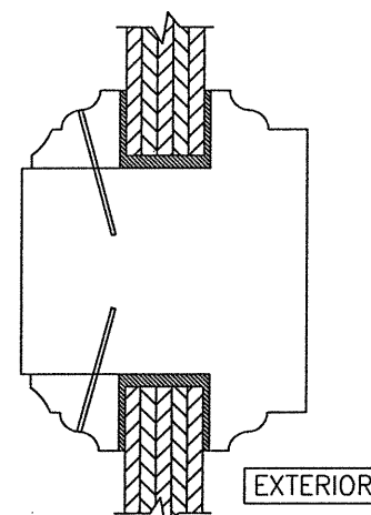
SECTION L SCALE: 1/2 FULL (WOOD PANEL OVER WOOD PANEL)
