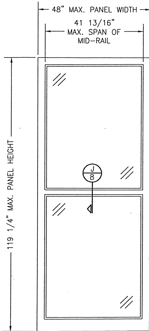
INTERIOR ELEVATION: ALL GLASS PANEL WITH MID-RAIL SCALE: 1/2" = 1'-0"
