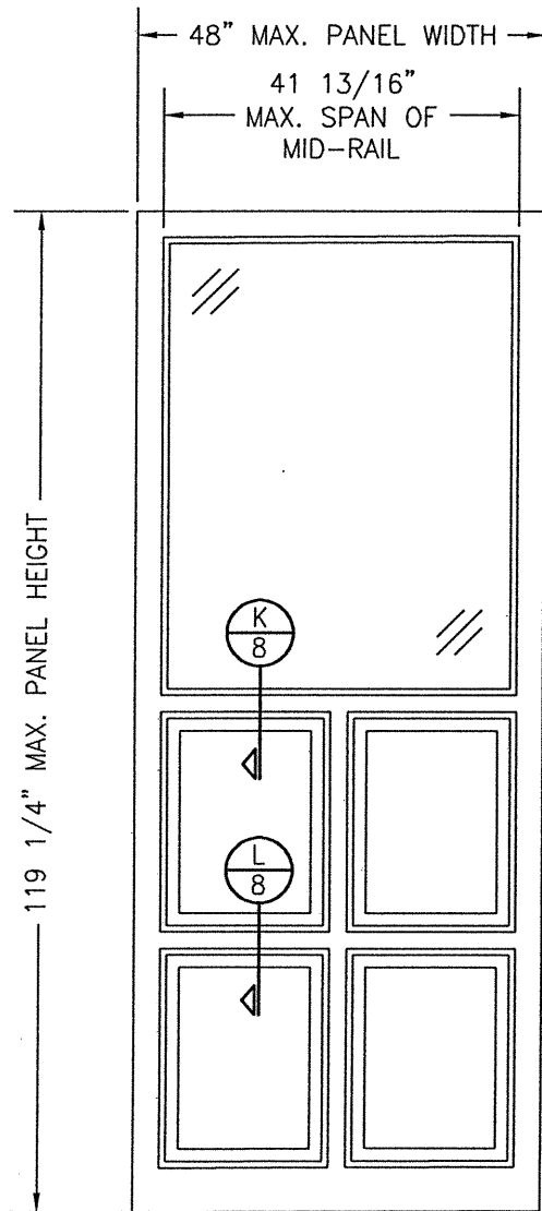
INTERIOR ELEVATION: PARTIAL WOOD PANEL WITH MID-RAIL SCALE: 1/2" = 1'-0"
