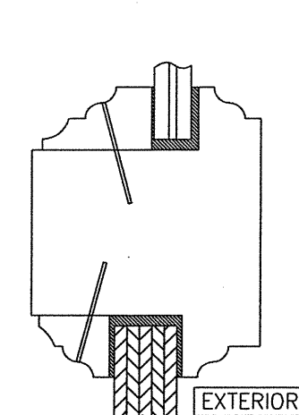
SECTION K SCALE: 1/2 FULL (GLASS OVER WOOD PANEL)
