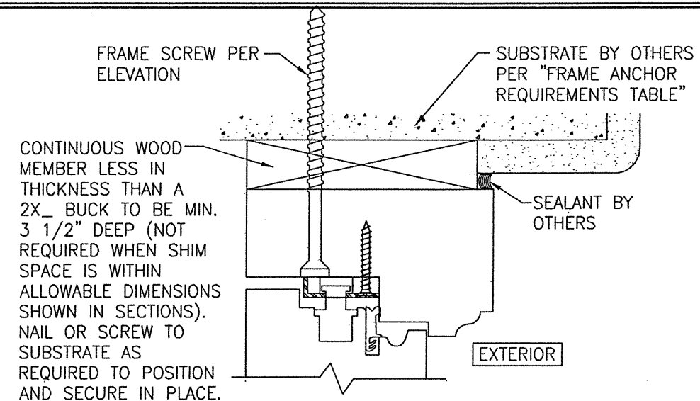
OPTIONAL DIRECT MOUNT DETAIL TO SUBSTRATE WITH SPACER (HEAD SECTION SHOWN; SILL & SIDES ARE INSTALLED THE SAME) (FOR DETAIL NOT SHOWN, SEE OTHER SECTIONS) (NOT APPLICABLE WITH FIXED PANEL DOORS)
