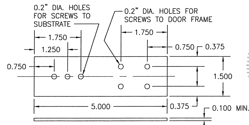
FLAT CLIP (STAINLESS STEEL OR GALVANIZED STEEL)
