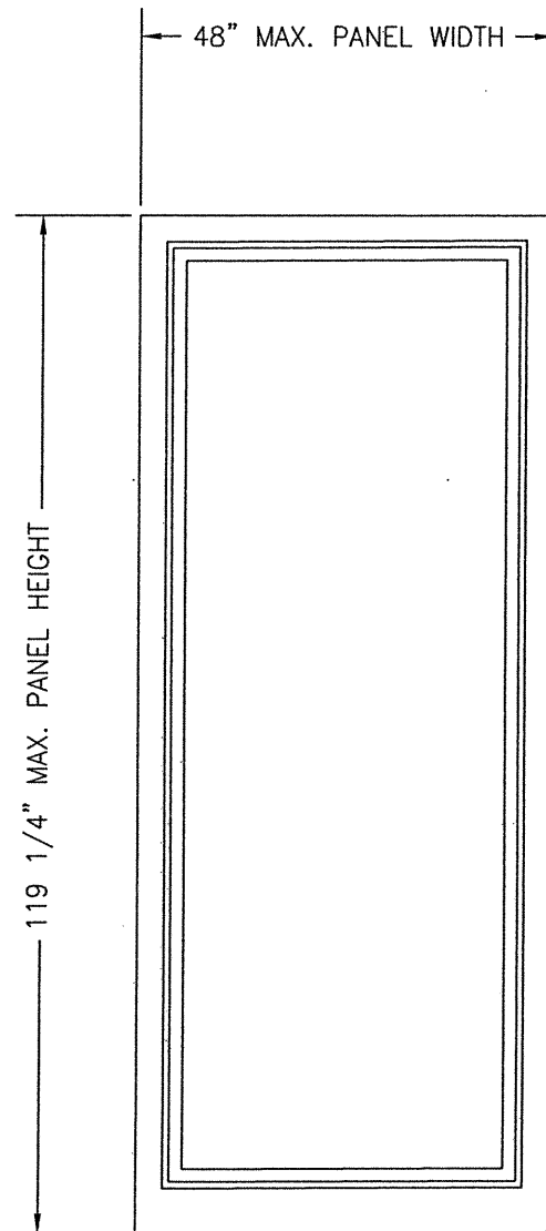
INTERIOR ELEVATION: FULL WOOD PANEL SCALE: 1/2" = 1'-0"
