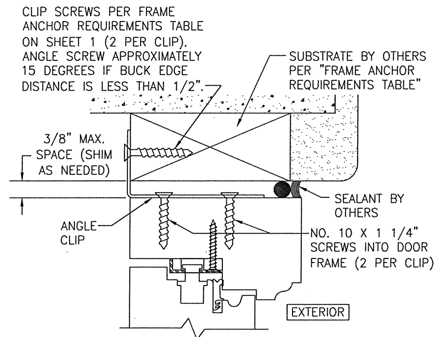
OPTIONAL ANGLE CLIP MOUNT DETAIL AT HEAD & SIDES (HEAD SECTION SHOWN. SIDES ARE INSTALLED THE SAME)
