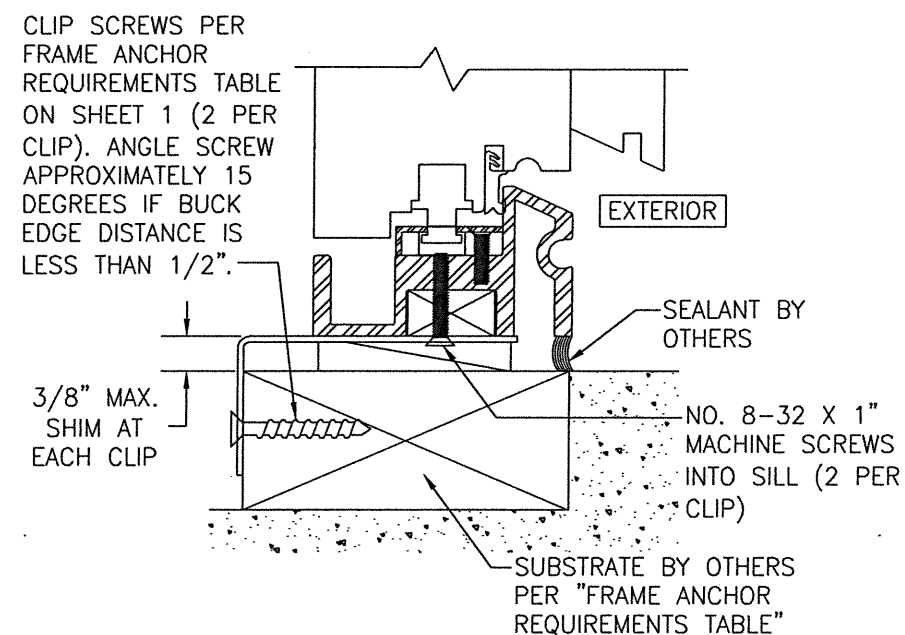
OPTIONAL ANGLE CLIP MOUNT DETAIL AT SILL
