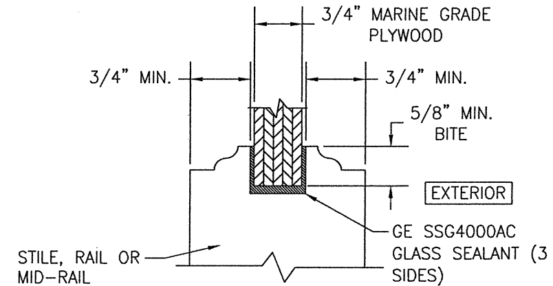
TYPICAL GLAZING DETAIL (OPTIONAL WOOD PANEL CONDITION)
