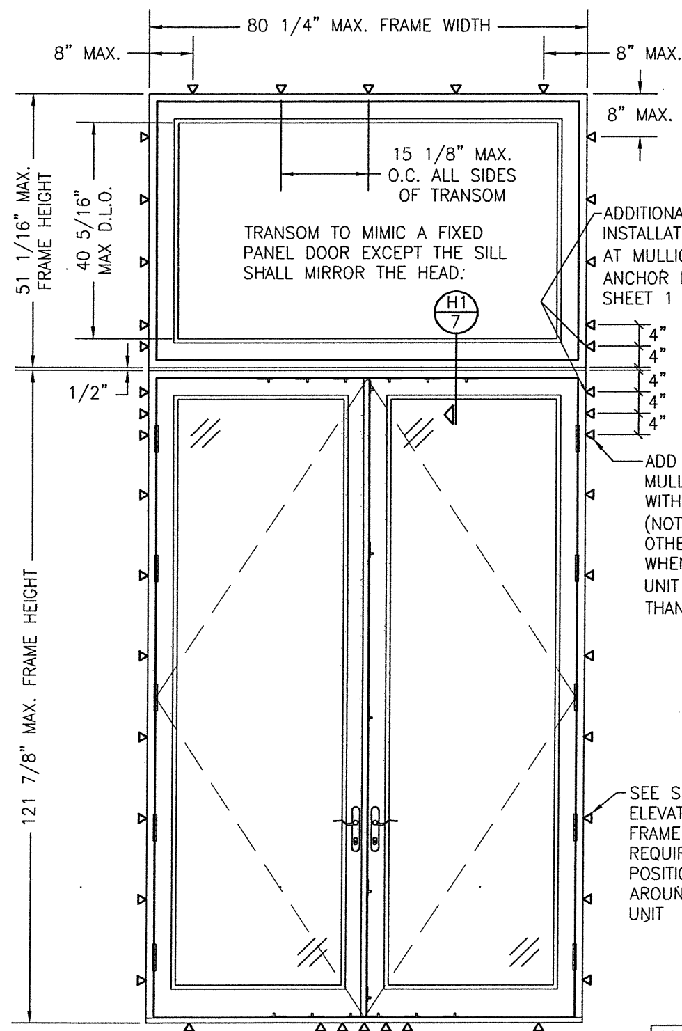
INTERIOR ELEVATION: DOUBLE DOOR WITH TRANSOM UNIT
