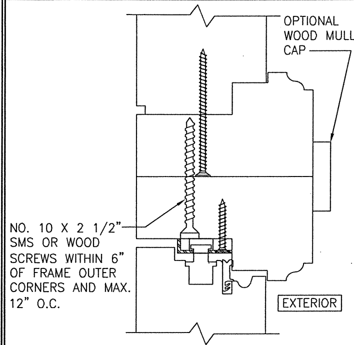
SECTION H2 SCALE: 1/2 FULL
