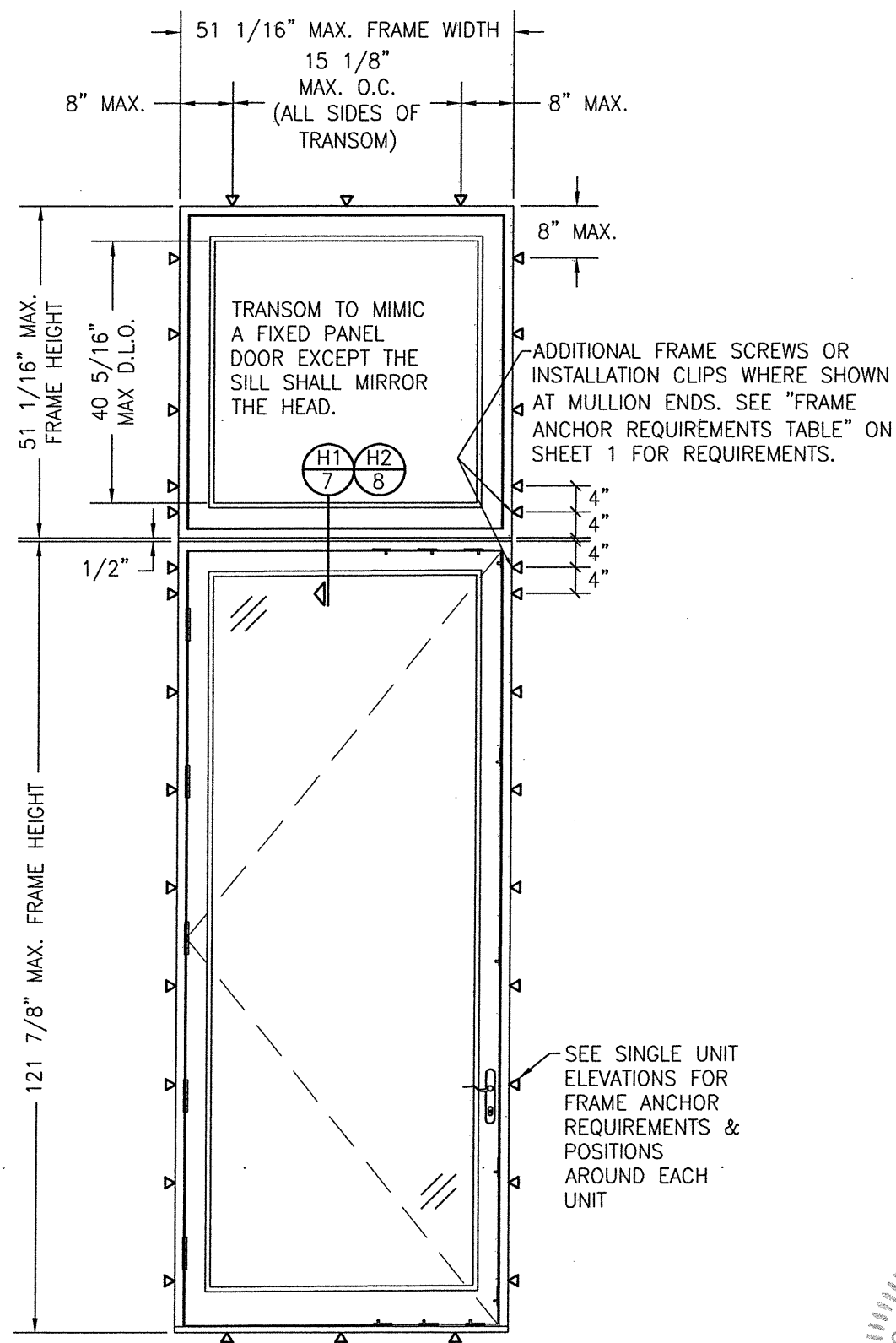
INTERIOR ELEVATION: SINGLE ACTIVE OR FIXED DOOR WITH TRANSOM UNIT
